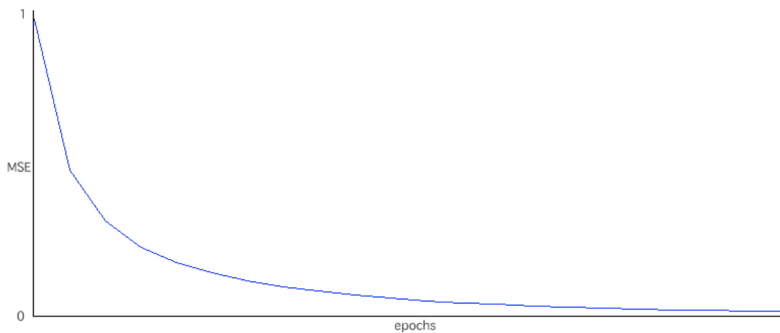
Figure 3.9: Training graph
